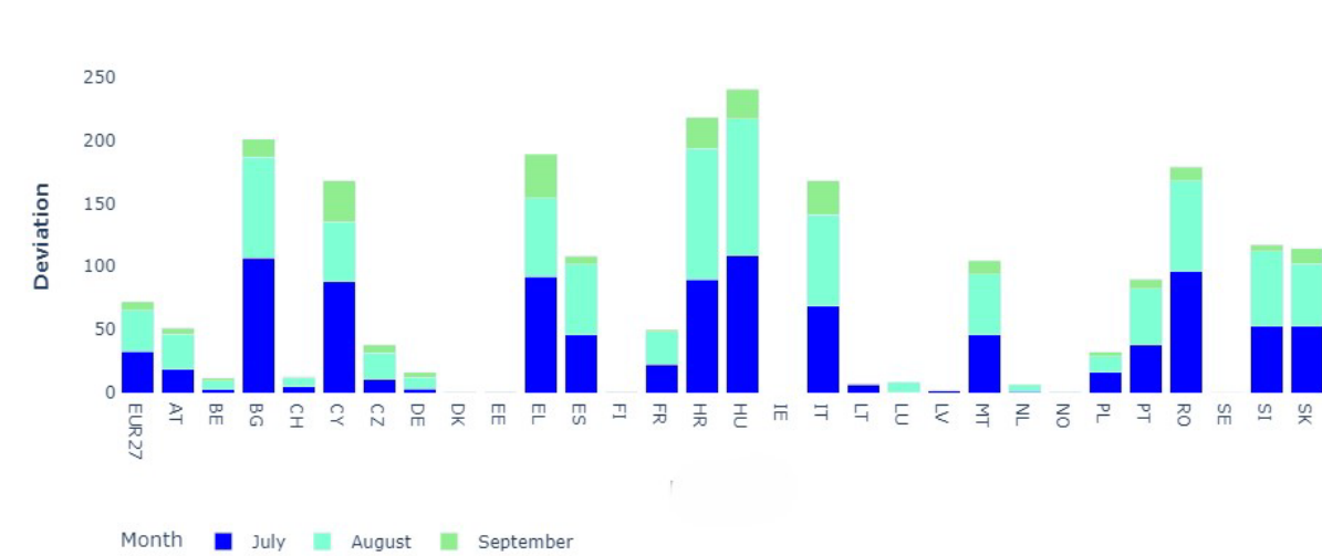
Figure 6 – Deviation of actual Cooling Degree Day (CDD) from the long-term average in Q3 of 2024
